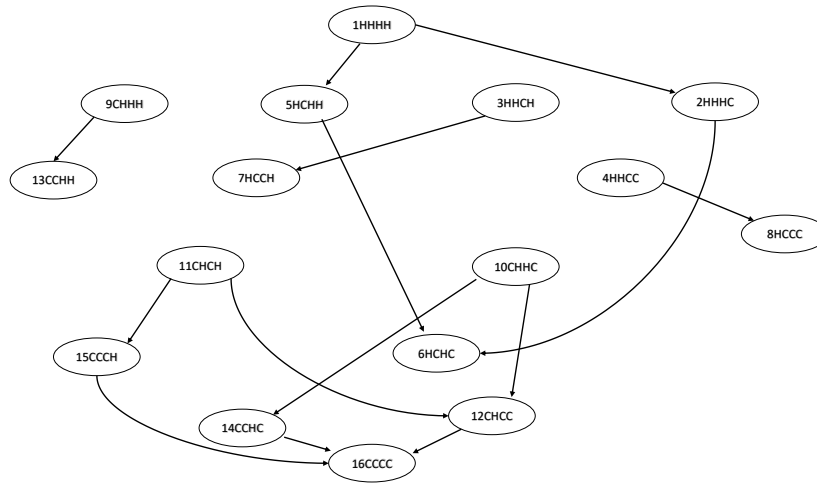
Figure 4: Graph illustrating restrictions with the p-values of the LR test greater than 0.01 obtained in case of diagonal contemporaneous covariance matrix (M0). CF measure: POR_IN
